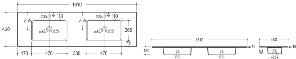
City 161x46cm 2s (80+80)
