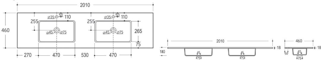
City 201x46cm 2s (100+100)
