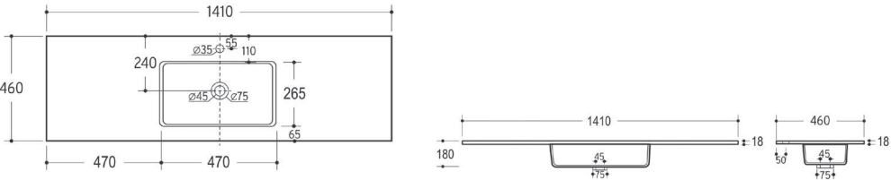
City 141x46cm 1s
