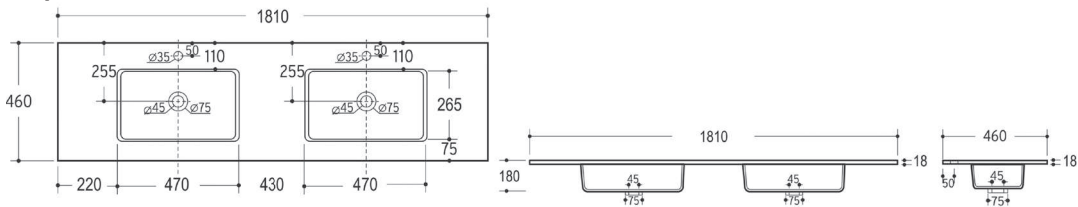
City 181x46cm 2s (90+90)
