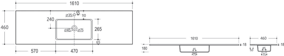
City 161x46cm 1s
