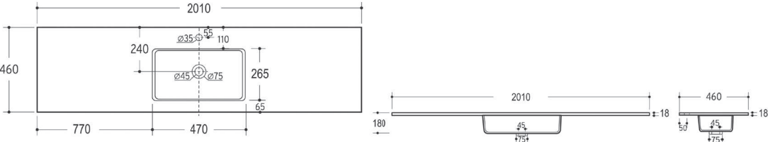
City 201x46cm 1s
