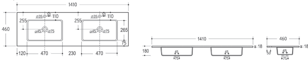
City 141x46cm 2s (70+70)
