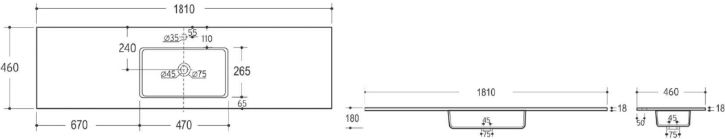
City 181x46cm 1s
